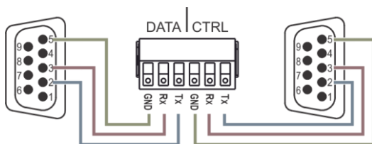
Figure 7: RS-232 Pinout
